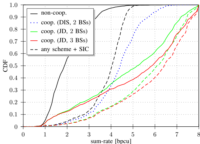
Fig. 5: CDF of sum-rates observed on the measurement route. used in the LTE-Advanced uplink.
