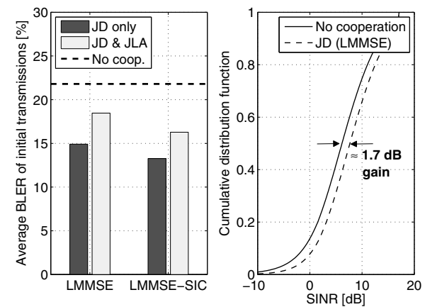
Fig. 3. Average BLERs of the initial transmission attempts for joint detection (JD) only as well as JD combined with joint link adaptation (JLA) and distribution of the SINR values after LMMSE equalization. All results are given for the Macro 1 case with proportional fair scheduling.
