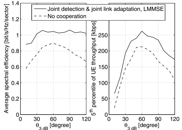
Fig. 5. Impact of the half-power beamwidth at the BS side on the system performance for the Macro 1 case with and without intra-site cooperation. In all cases, P-FR scheduling with HARQ is assumed.
