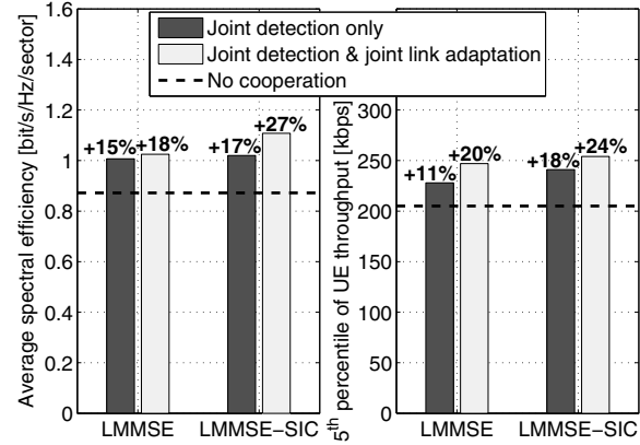
Fig. 1. Performance of joint detection as well as joint link adaptation for proportional fair scheduling with HARQ and two different receiver types for the Macro 1 case. The given percentages denote the relative performance gains compared to the reference case without any cooperation.
