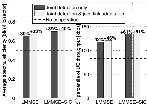
Fig. 4. Performance of intra-site cooperation for RR scheduling w/o HARQ and the Macro 1 case. The given percentages denote the relative performance gains over the reference case without any cooperation.
