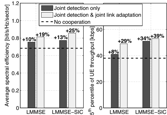
Fig. 2. Performance of joint detection as well as joint link adaptation for proportional fair scheduling with HARQ and two different receiver types for the Macro 3 case. The given percentages denote the relative performance gains compared to the reference case without any cooperation.
